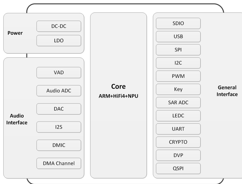
Fig. 2.1 Block Diagram
